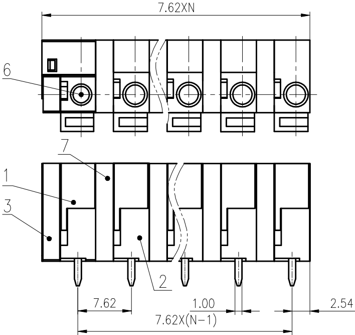
PCB LAYOUT 7.62X(N-1)
