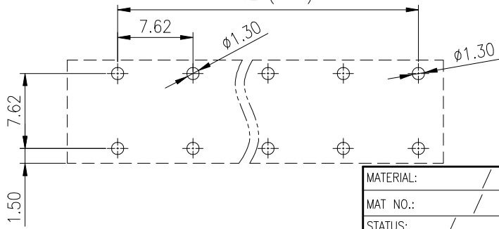
PCB LAYOUT 7.62X(N-1)
